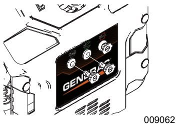
Figure 2-5. Insert Nozzles
