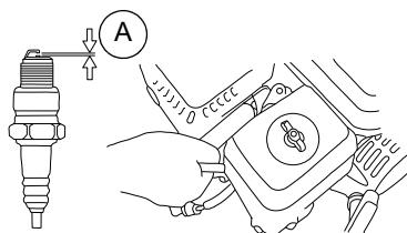
Figure 4-8. Bougie
