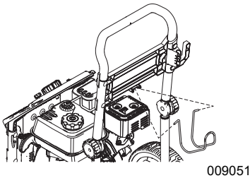
Figure 2-4. Install Hose Hook
