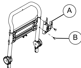
Figure 2-2. Install Gun Hook
