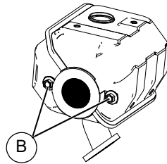
Figure 4-10. Spark Arrestor Fasteners
