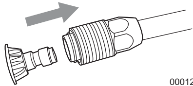
Figure 2-16. Insertion de la buse
