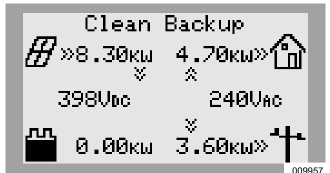
Figura 7-26. Clean Backup (Reserva limpia) (2 de 2)
