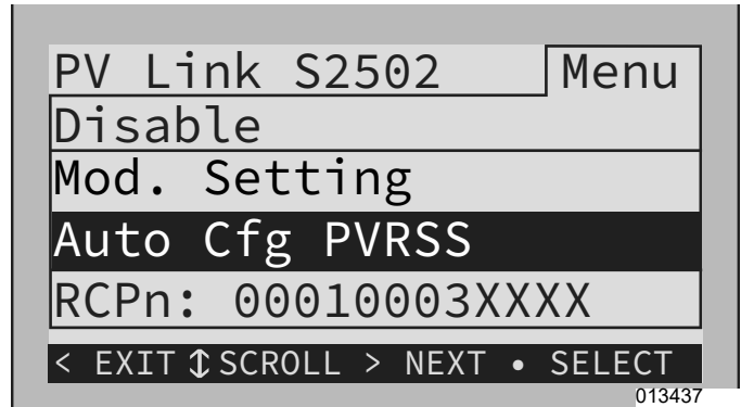
Figura 7-14. PV Link: Auto Cfg PVRSS
